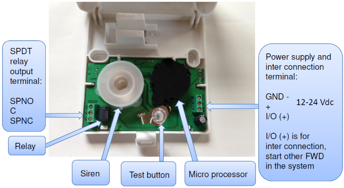
PCB for Room Smoke Detector with Fire Alarm Siren and Relay Output FWD 305
